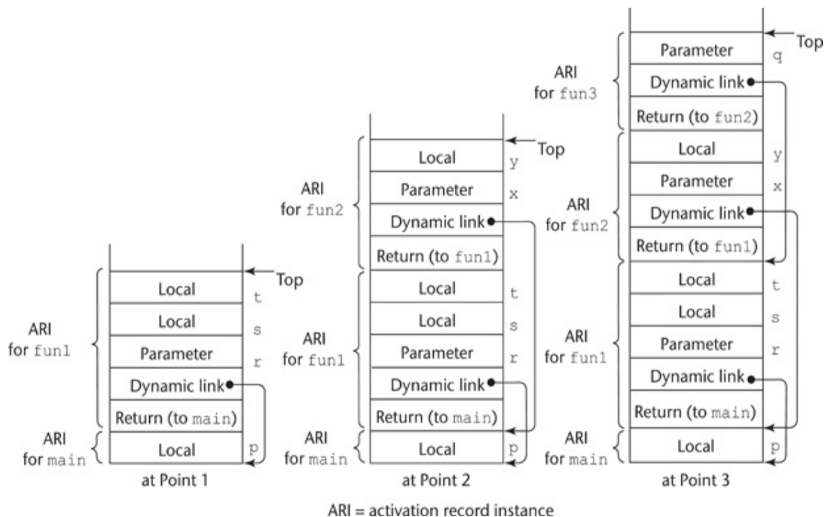
Figure 10.5 Stack contents for three points in a program
