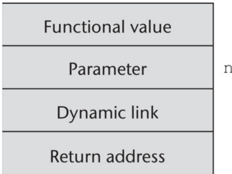
Figure 10.6 The activation record for factorial
