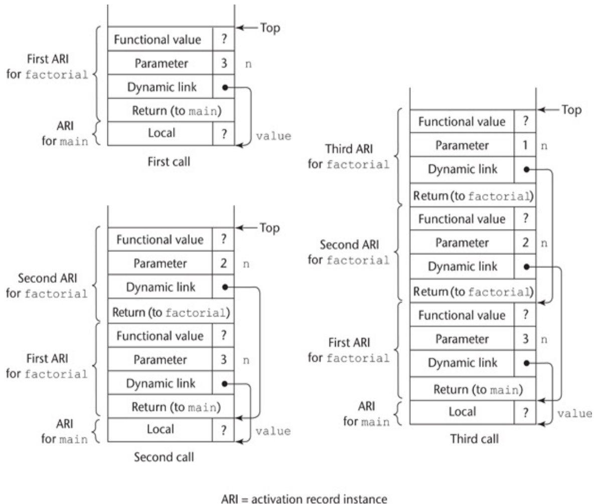
Figure 10.7 Stack contents at position 1 in factorial
