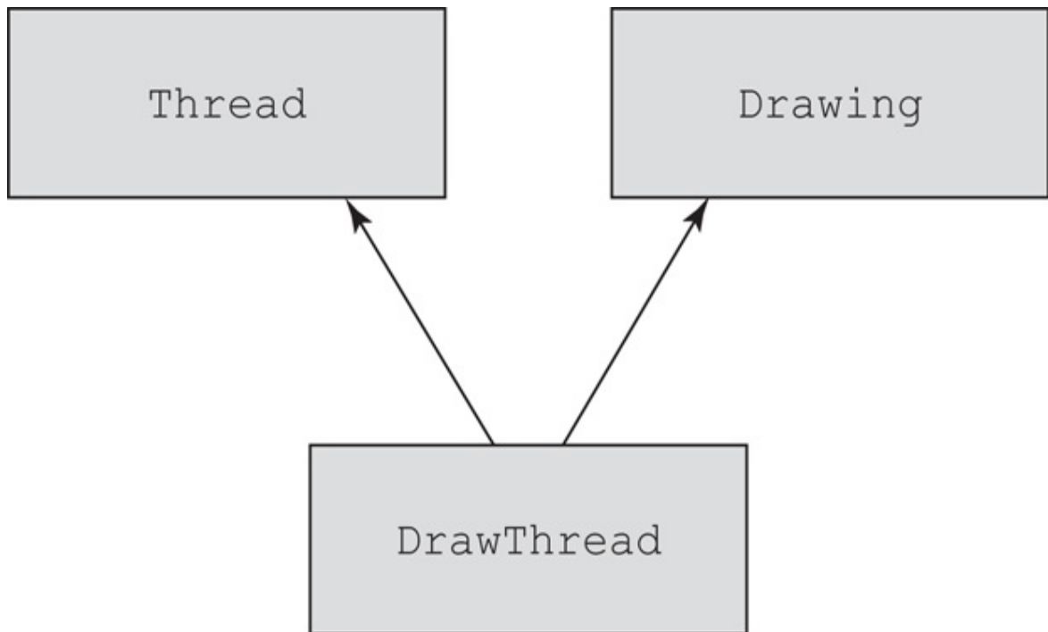
Figure 12.5 Multiple inheritance
